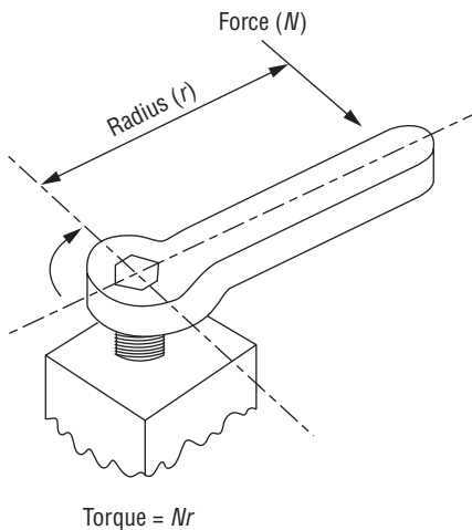
Fig. 2.5 Torque
