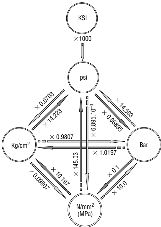
Fig. 2.2 Pressure conversions
