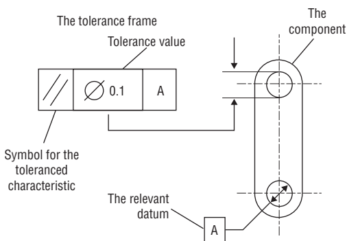
Fig. 12.4 Tolerancing symbols
